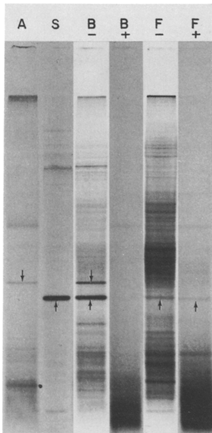
FIGURE 7 Analysis by SDS-PAGE and AR of products synthesized at the 120-min time point as described in Fig. 6 after incubation in the absence or presence of proteolytic enzymes. Shown are the labeled products synthesized in an initiation system in the presence of light chain mRNA (slot A), the labeled secreted light chain (slot S), and the products synthesized in a readout system containing detached ribosomes (slot B-) subsequently subjected to proteolysis (slot B+) or containing crude free ribosomes (slot F-), subsequently subjected to proteolysis (slot F+). Symbols used were as in Fig. 5.
