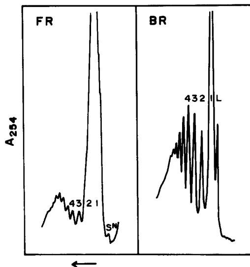
FIGURE 1 Sedimentation profile of free (FR) and detached (BR) ribosomes from MOPC 41 DL-1. Pellets of free and detached ribosomes were resuspended in ice-cold double-distilled water. 0.2-ml aliquots containing 3.0 A_{254} units were layered on 12.5 ml of 10-40% sucrose gradients in 100 mM KCl, 20 mM triethanolamine-HCl pH 7.4 at 20°C, and 3 mM MgCl_2 . The gradients were centrifuged at 4°C in an SB 283 rotor of an IEC centrifuge for 100 min at 190,000 g_{av} . Fractionation of the sucrose gradients and recording of the optical density were as described (6). Arrow indicates direction of sedimentation. The native small ribosomal subunit peak is designated as S^N , the large ribosomal subunit peak as L, the mono-, di-, tri-, and tetrasome peaks, as 1, 2, 3, and 4, respectively.
