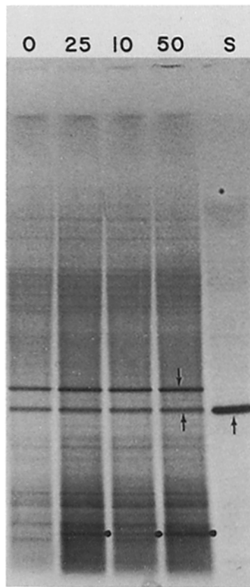
FIGURE 11 Analysis by SDS-PAGE and AR of the products synthesized at 120-min time point as described in Fig. 10. Slot numbers refer to microliters of S^N present in the readout system with detached ribosomes (see Fig. 10). For comparison, the labeled secreted light chain of IgG is included in slot S. Symbols used were as in Fig. 5
