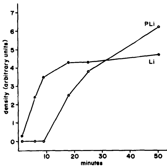
FIGURE 9 Quantitation by densitometry of the autoradiograph shown in Fig. 8. PLi and Li designate the unprocessed (downward pointing arrow in Fig. 8) and the processed light chains of IgG (upward pointing arrow in Fig. 8), respectively.
