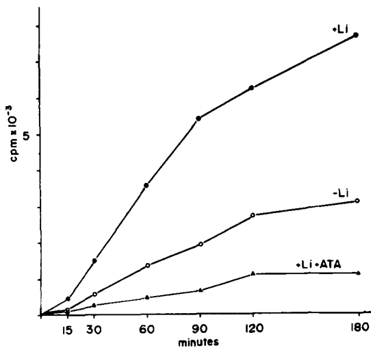
FIGURE 4 Time-course of polypeptide synthesis in an initiation system in the presence of mRNA for the light chain of IgG (+Li), in the presence of light chain mRNA and of 10^{-4} M ATA (+Li + ATA), and in the absence of mRNA (-Li). For details, see Materials and Methods.
