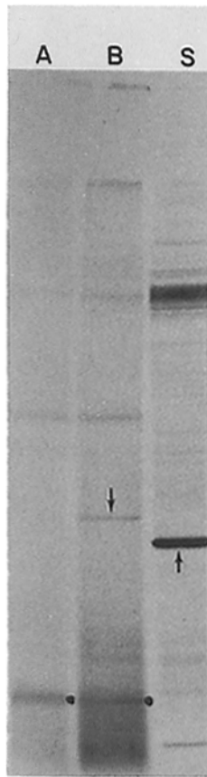
FIGURE 5 Analysis by SDS-PAGE and AR of an experiment of the type described in Fig. 4. Shown are the labeled products synthesized at the 180-min time point in the absence of mRNA (slot A) or in the presence of mRNA for the light chain of IgG (slot B). For comparison the labeled secreted light chain of IgG is shown in slot S (upward pointing arrow). Downward pointing arrow (slot B) indicates precursor of the light chain of IgG. Dots indicate the globin chains.
