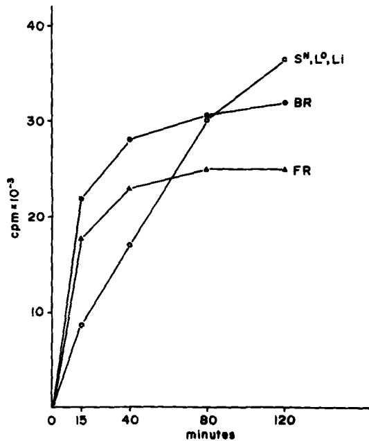
FIGURE 6 Time-course of polypeptide synthesis in a readout system containing 9.8 A_{260} units of crude free (FR) or 5.4 A_{260} units of detached (BR) ribosomes. For comparison the time-course of polypeptide synthesis in an initiation system containing mRNA for the light chain of IgG ( S^N , L^O , Li) was included. In the latter case, 50- \mu l aliquots were counted, whereas in the former 10- \mu l aliquots were counted.
