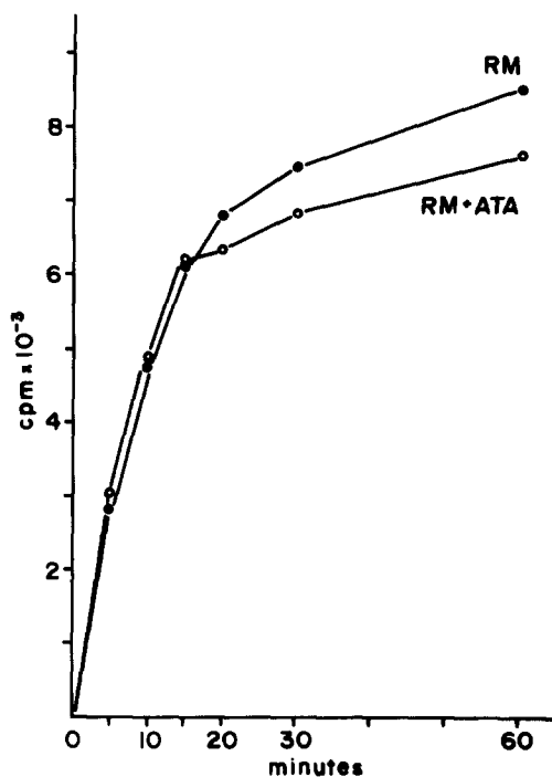
FIGURE 13 Time-course of polypeptide synthesis in the absence of ATA (RM) or presence (RM+ATA) of 10^{-4} M ATA in a readout system containing rough microsomes ( 4.3 A_{260} units).
