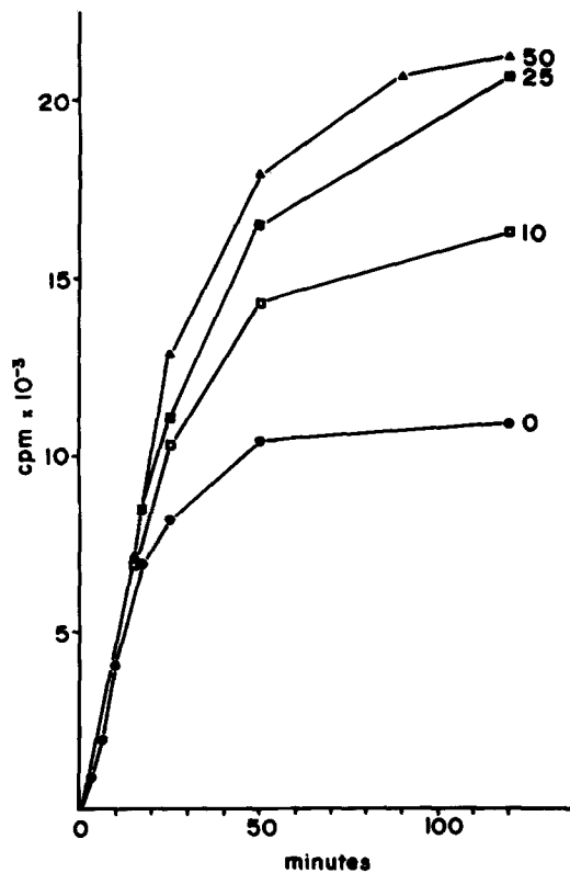
FIGURE 10 Time-course of polypeptide synthesis in a readout system containing detached ribosomes ( 1.8 A_{260} units) and S^N from reticulocytes as a source for initiation factors. Numbers next to curves designate the amount (in microliters) of S^N ( 10.5 A_{260} units/ml) present in the 250\text{-}\mu\text{l} assay.
