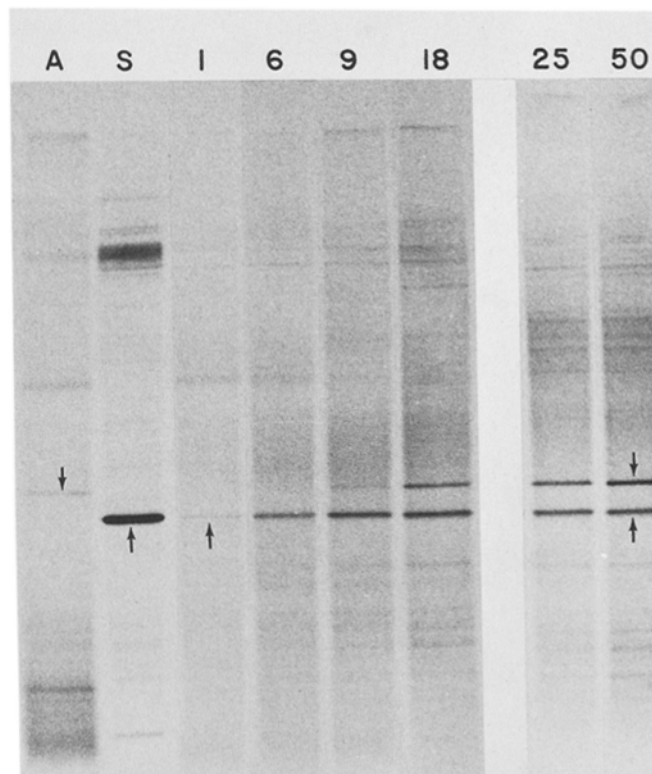
FIGURE 8 Analysis by SDS-PAGE and AR of the products synthesized by detached ribosomes ( 1.8 A_{260} units) during the course of readout in the presence of 10^{-4} M ATA. Readout was terminated at 1, 6, 9, 18, 25, and 50 min (slots 1, 6, 9, 18, 25, 50, respectively) by cooling 25\text{-}\mu\text{l} aliquots to 0^{\circ}\text{C} and adding 25\ \mu\text{l} 20% TCA. For comparison, the precursor of the light chain (slot A) synthesized in an initiation system (see Fig. 5) and the labeled secreted light chain (slot S) were included. Symbols used were as in Fig. 5. Slots 25 and 50 were from a separate slab gel.
