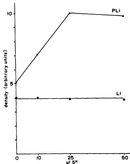
FIGURE 12 Quantitation by densitometry of autoradiograph shown in Fig. 11. PLi and Li designate the unprocessed and processed chains of IgG, respectively.
